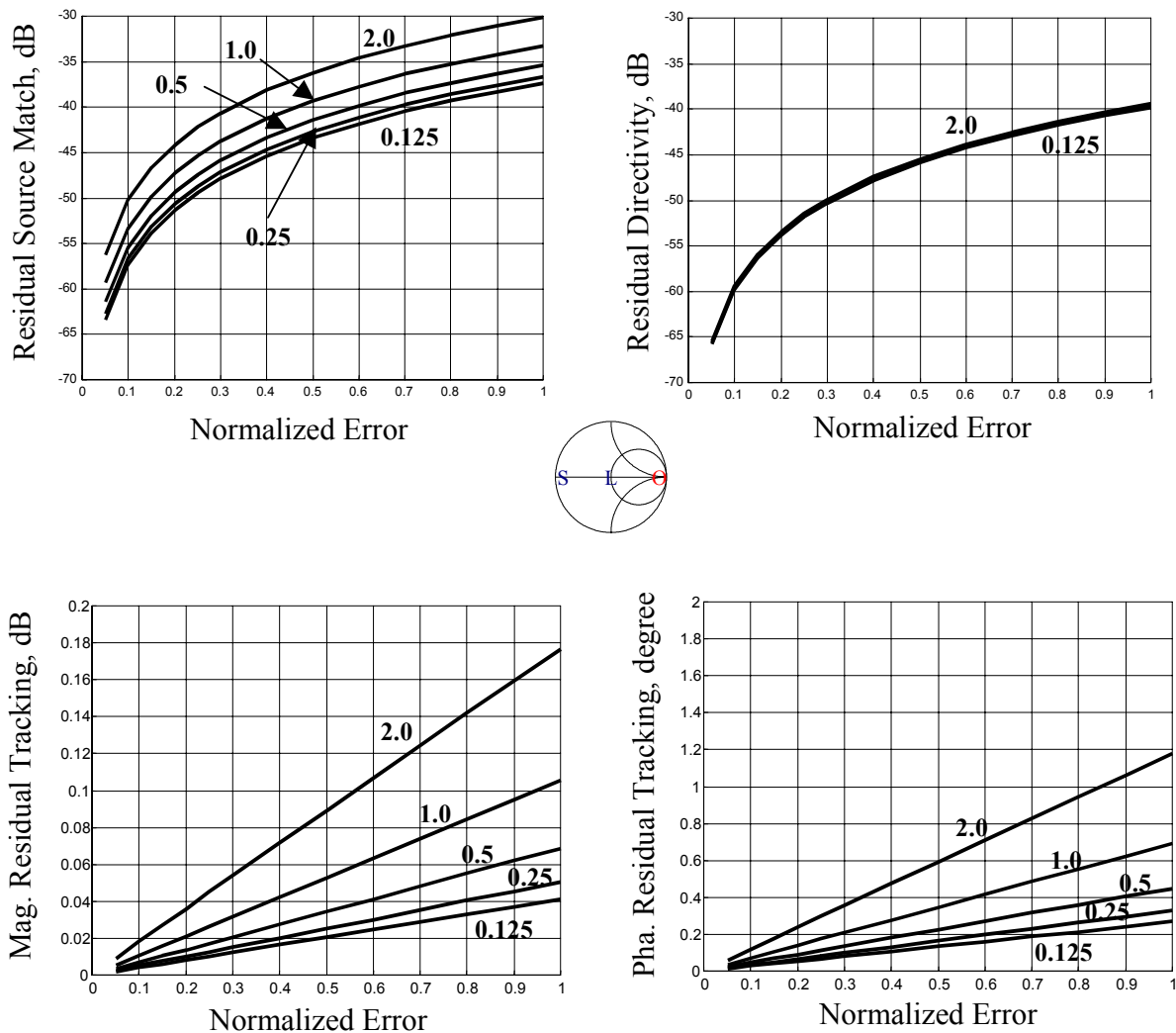
Figure 6. Sensitivity of error in model data used for the open. Five different values of \max(|\Delta\Gamma_O|) , in terms of degrees in phase, 2.0, 1.0, 0.5, 0.25, 0.125, are considered.
