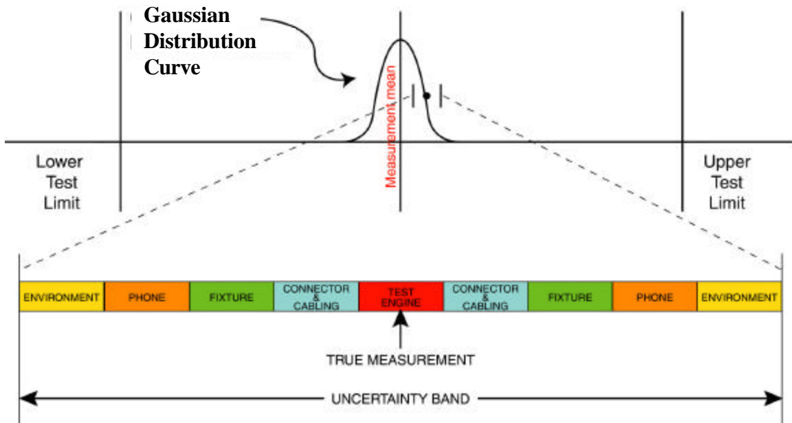
Figure 1. Measurement uncertainty.
