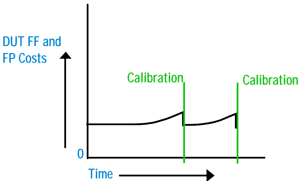
Figure 9. Calibration effects.
